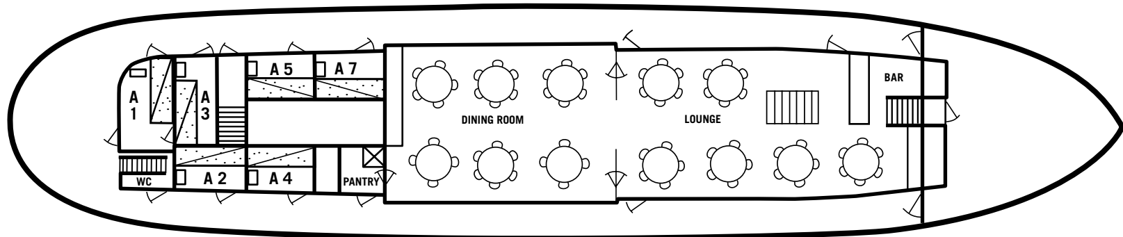
SHELTER DECK
