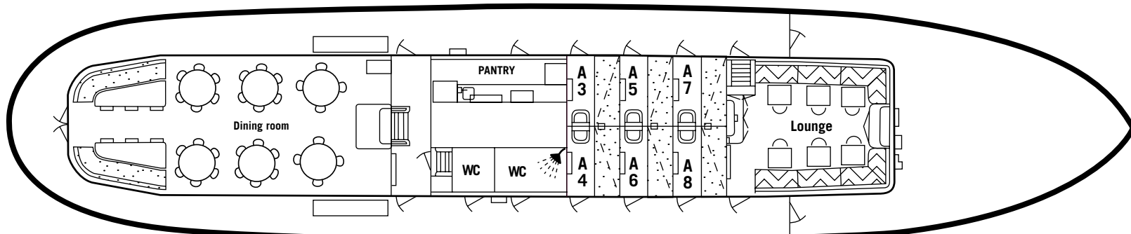
SHELTER DECK
