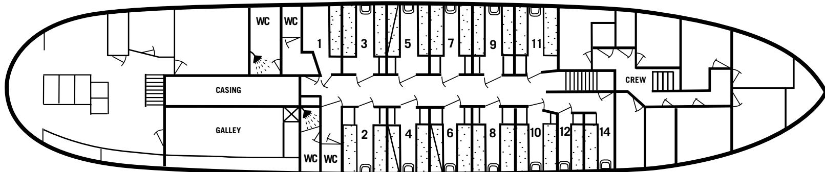
MAIN DECK
