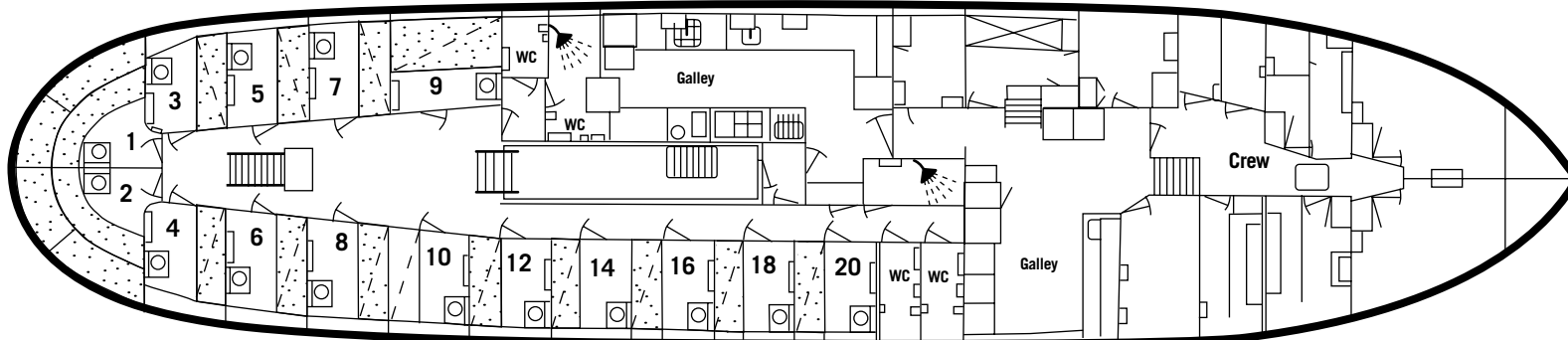
MAIN DECK
