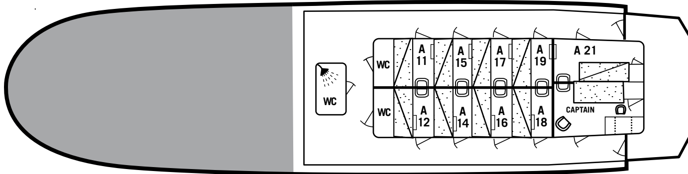
SHELTER DECK
